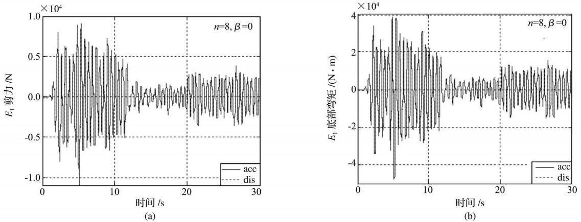
图 6 E_1 剪力和弯矩比较 ( n = 8, \beta = 0 )
